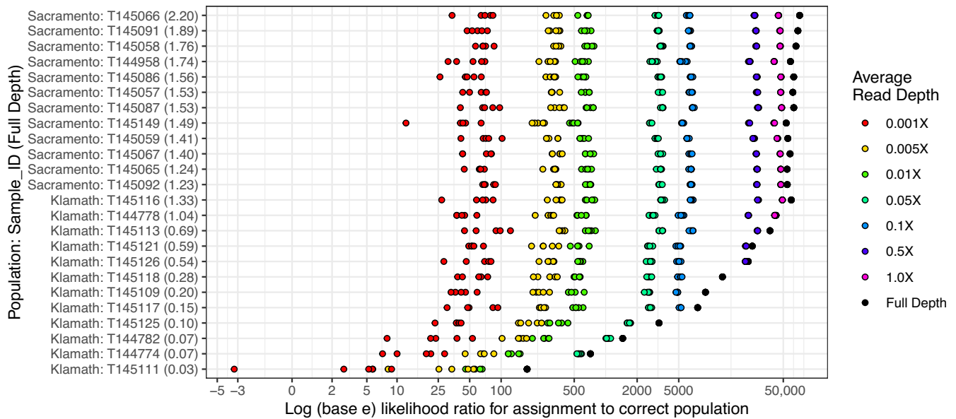
FIGURE 6 Log-likelihood ratios for assignment at different read depth levels for the Chinook salmon data. On the y-axis are different Chinook salmon samples, labelled by their population, a colon, their ID number and then in parentheses the average read depth of their aligned data at full depth. On the x-axis is the log-likelihood ratio in favour of assignment to their own (correct) population on a 'pseudo-log' scale that accommodates negative values. Positive numbers indicate correct assignment. Colours denote the read depths after downsampling. There are five points for each individual at each value of downsampling, reflecting the five different seeds used for downsampling.
